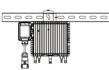
M60/80/100 G4 (2MPPTs) 安装
