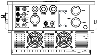
SUN-12/15K-SG01HP3-EU-AM2
